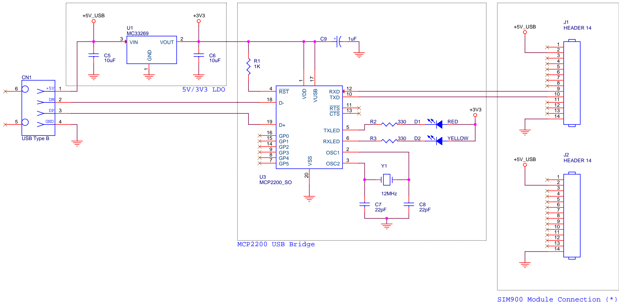
SIM900 Module Connection (*)
