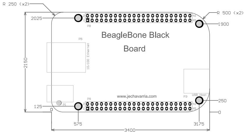
Outline Dimensions (Official) All dimensions in mils
