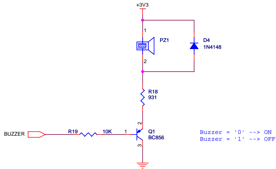
Buzzer
