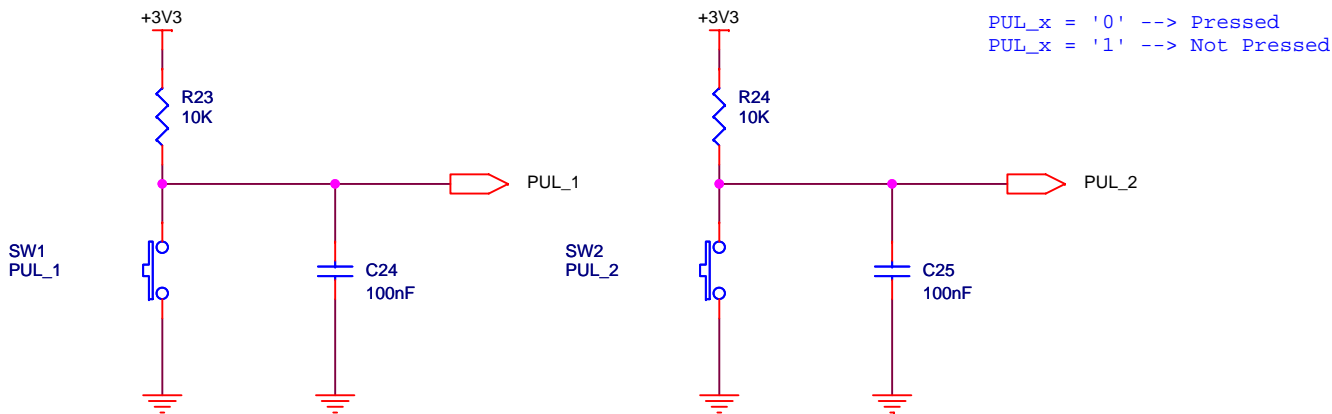
Pushbuttons
